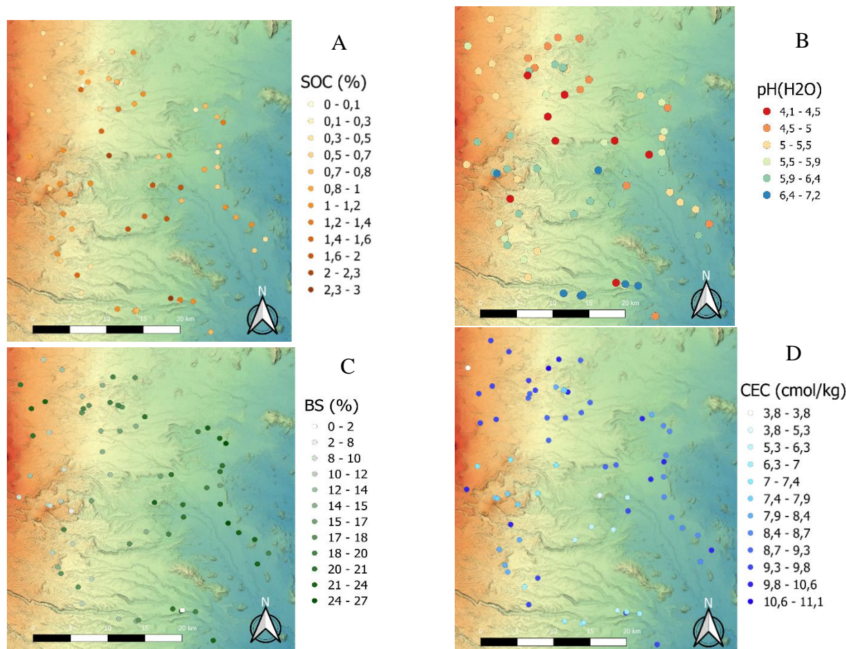
Figure 4.1. Soil property maps for selectected attributes: soil organic carbon (A), pH (B), Base saturation (C) and Cation exchange capacity (D)
